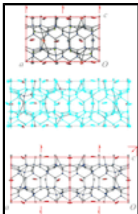
Fig. 4. Comparison between the '3331' P112_1 (top) and '5551' Pmn2_1 (bottom) structures projected along the b axis. Superposition of 3331 (blue) onto 5551 is shown in the middle where the screw axis at x=0 in 3331 overlaps with that at x=0.25 in 5551.
