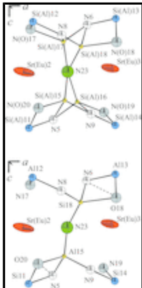
Fig. 3. Local structure around the Si(Al)15-16 and Si(Al)17-18 split pairs in the sechser ring layer (top), and one of the possible conformations (bottom). The shared edge of tetrahedra is shown in dashed line in the bottom figure.
